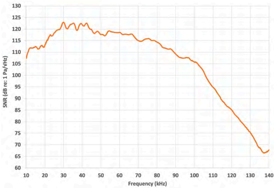
Figure 9. Ultrasonic Microphone Signal-to-Noise Ratio
