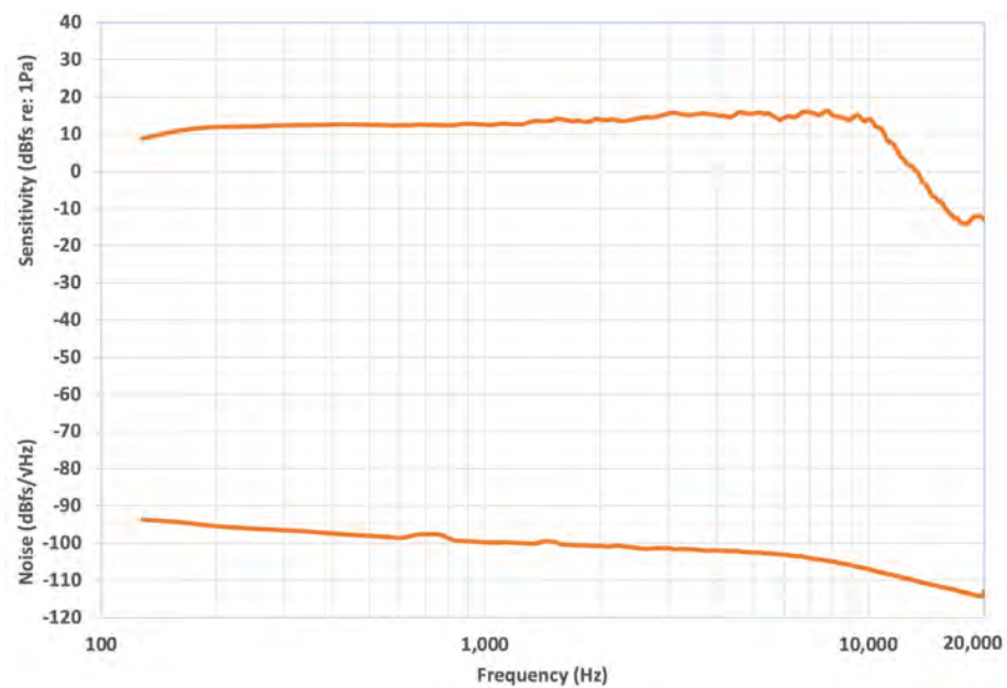
Figure 13. Sensitivity and Noise Floor, Logarithmic Frequency Scale
