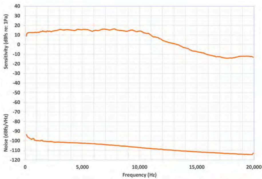
Figure 12. Sensitivity and Noise Floor, Linear Frequency Scale
