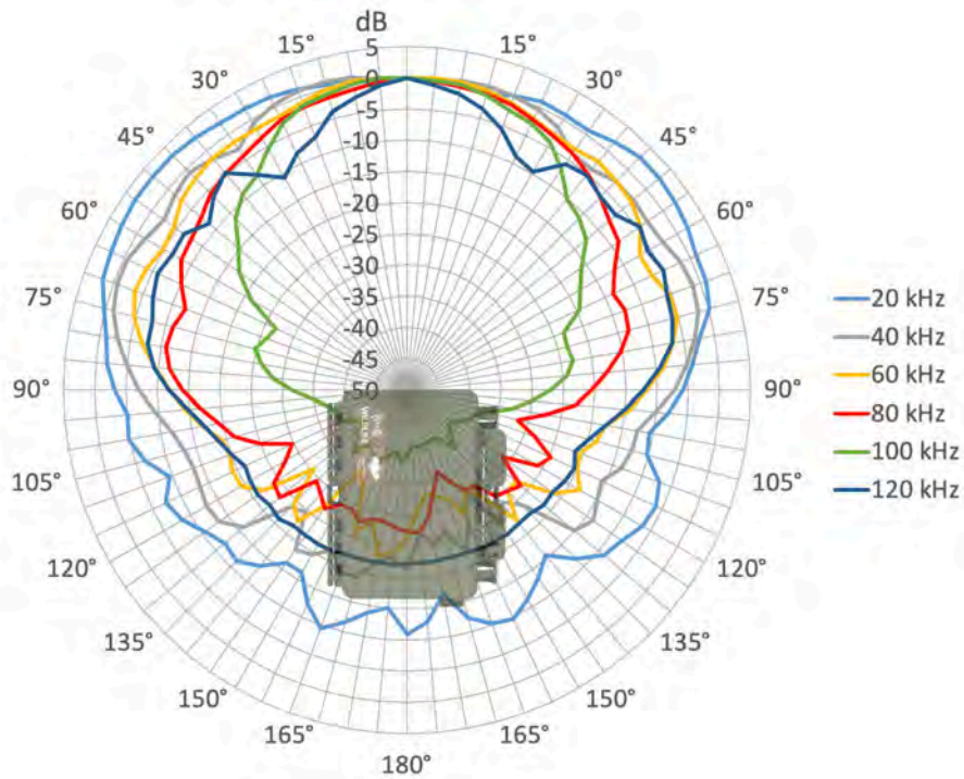
Figure 11. Ultrasonic Microphone Polar Response: Top View
